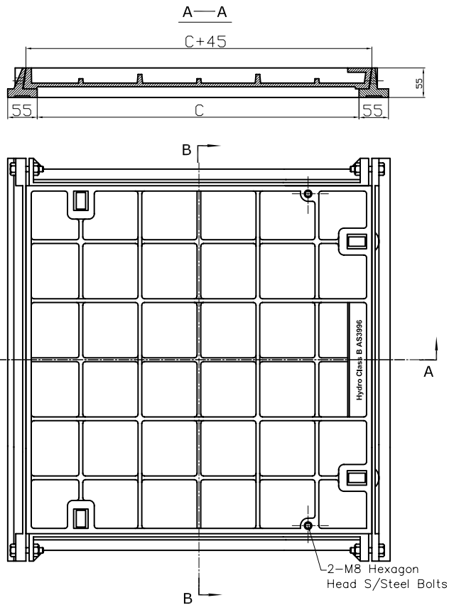
Bolt Hole Profile
